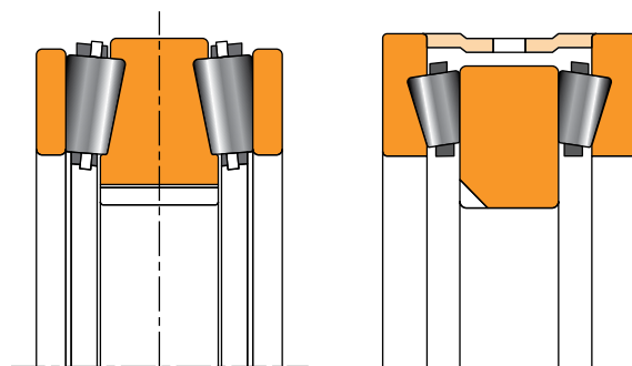
Fig. 95. TTDWK assembly (with flat outer washers).
