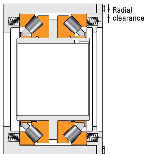
Fig. 94. Double-directional 2TSR.
