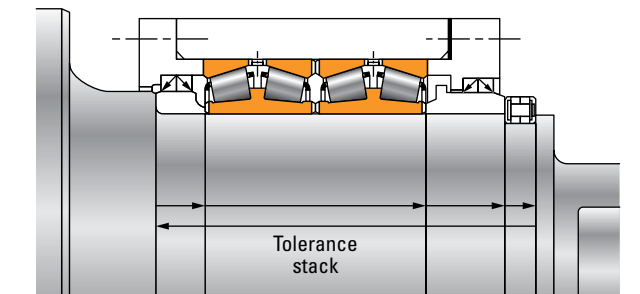
Fig. 244. Non-adjustable retaining design.
